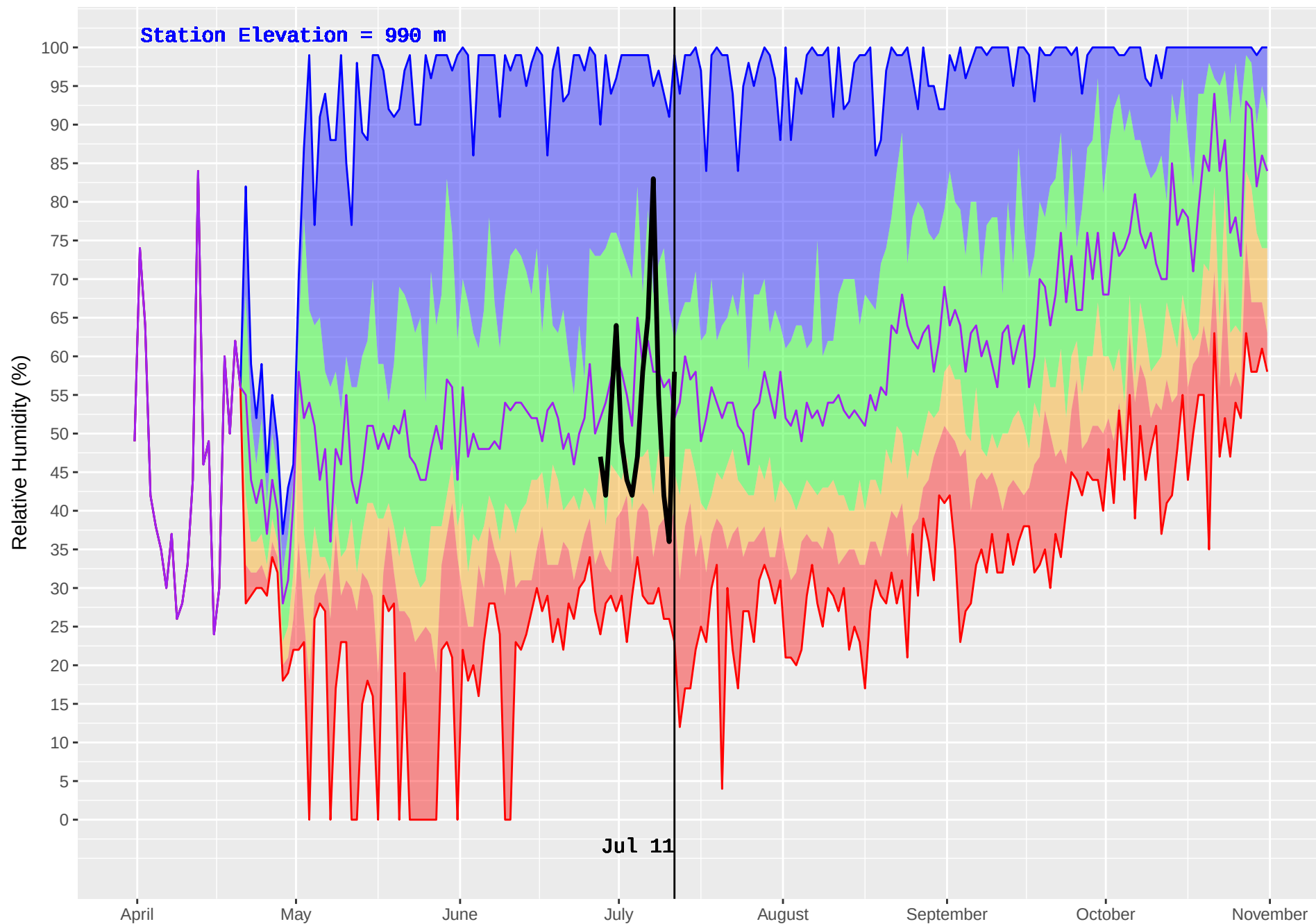
LOVELL COVE (163) : Historical (1979–2016) and Current (2018) Noon Relative Humidity
