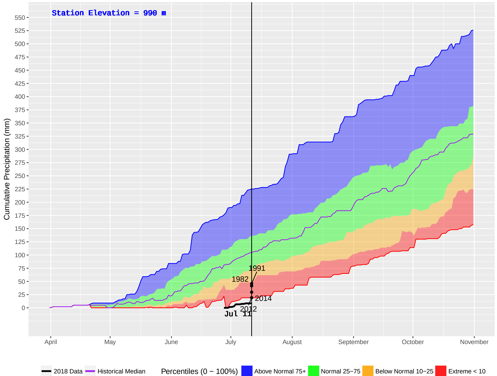
LOVELL COVE (163) : Historical (1979–2016) and Current (2018) Noon Cumulative Precipitation
